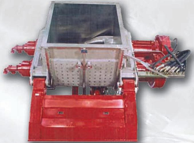
2800 Liter Mixer with Hydraulic Drive and Cored Blades Supplied for the manufacture of Ink Flushes
