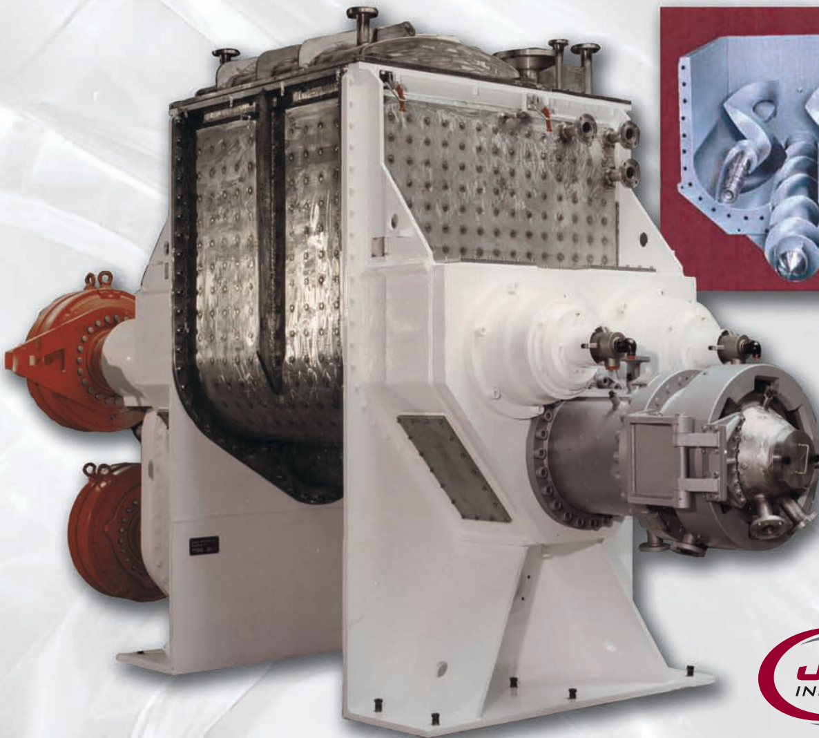
3800 Liter Mixer Extruder with Hydraulic Drive Supplied for the manufacture of Industrial Silicones
