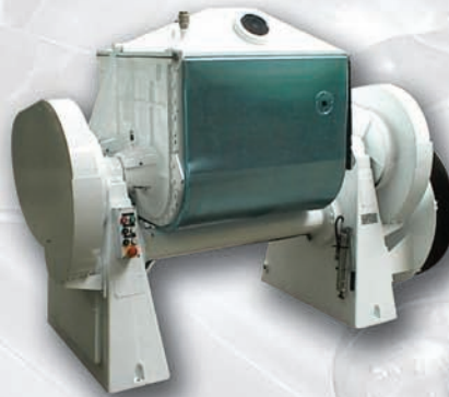
Rebuilt 350 Liter Mixer Supplied for the manufacture of Candy and Food Products
