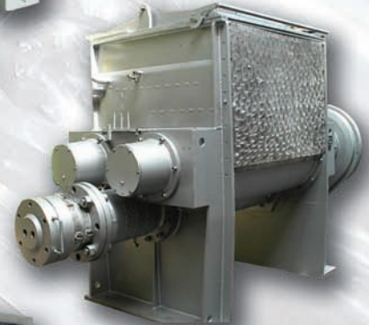
Rebuilt 660 Liter Mixer Extruder supplied for the manufacture of Run-Flat Tire Sealant
